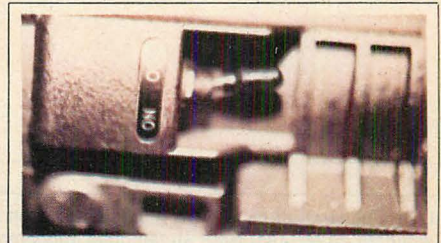
In keeping with streamlined concept, typical Starlight (passive) houses off-on switch in small, shielded receptacle on left side of telescope body. Is thus easily operated, yet protected from potential damage during field handling.
